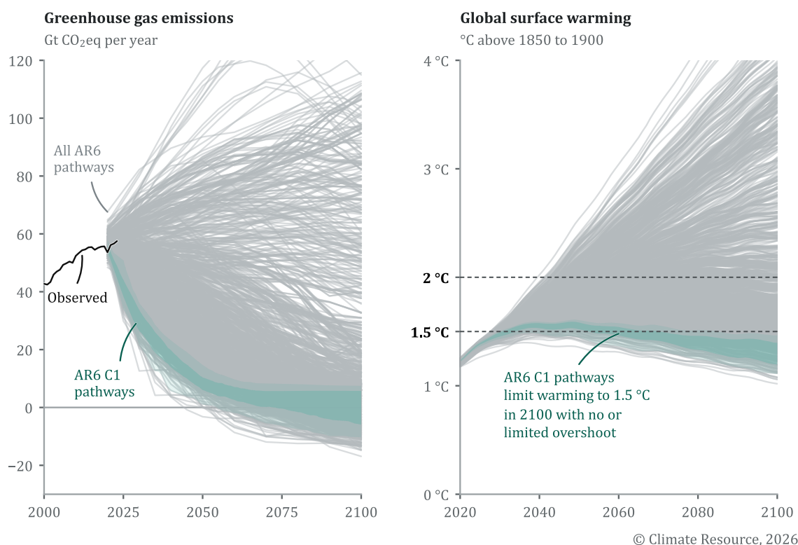
Figure 1: Greenhouse gas emissions (a) and global surface warming (b) in the 1,202 AR6 pathways (grey lines) and the 97 C1 pathways (interquartile and 5th–95th percentile ranges), with observed emissions to 2023 (black). Source: Byers et al. (2022); Nicholls et al. (2025); Climate Resource calculations. 12
