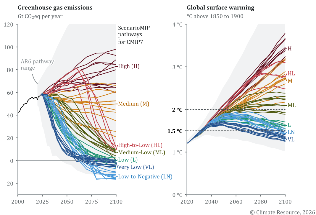
Figure 5: Greenhouse gas emissions (left) and global surface warming (right) in the 68 ScenarioMIP-CMIP7 pathways, coloured by category, against the range of the 1,202 AR6 pathways (grey) and observed emissions to 2023. Source: Riahi et al. (2026a); Byers et al. (2022); Nicholls et al. (2025); Climate Resource calculations. 24
