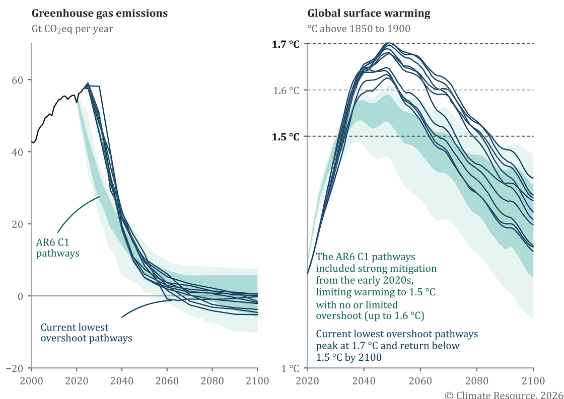
Figure 6: Greenhouse gas emissions (left) and global surface warming (right) in the ten current lowest-overshoot ScenarioMIP-CMIP7 pathways (lines) and the AR6 C1 pathways (interquartile and 5th–95th percentile ranges), with observed emissions to 2023. Source: Riahi et al. (2026a); Byers et al. (2022); Nicholls et al. (2025); Climate Resource calculations. 25
