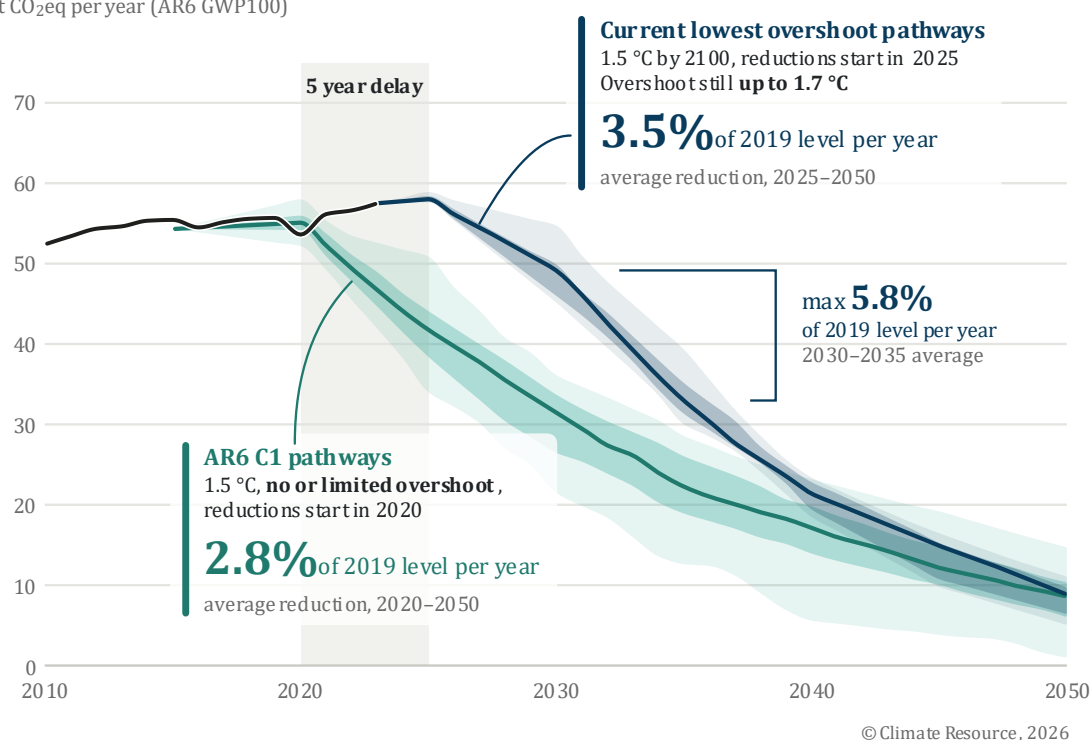
Figure 4: Greenhouse gas emissions in the AR6 C1 pathways and the ten current lowest-overshoot pathways (medians, interquartile and 5th–95th percentile ranges), and observed emission to 2023. Annual average emissions reductions are shown as a percentage of 2019 emissions. The steepest five-year reduction in the lowest-overshoot median (2030–2035) is also shown. Source: Byers et al. (2022); Riahi et al. (2026a); Nicholls et al. (2025); Climate Resource calculations. 22
