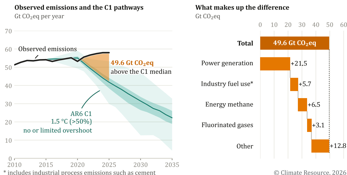
Figure 2: Observed greenhouse gas emissions and the AR6 C1 pathways (median, interquartile and 5th–95th percentile ranges), and the sources of the 49.6 Gt CO 2 eq by which observations exceeded the C1 median over 2020–2025. Source: Byers et al. (2022); Gütschow and Pflüger (2026); Crippa et al. (2026); Friedlingstein et al. (2026); IEA (2026e); Climate Resource calculations. 13
