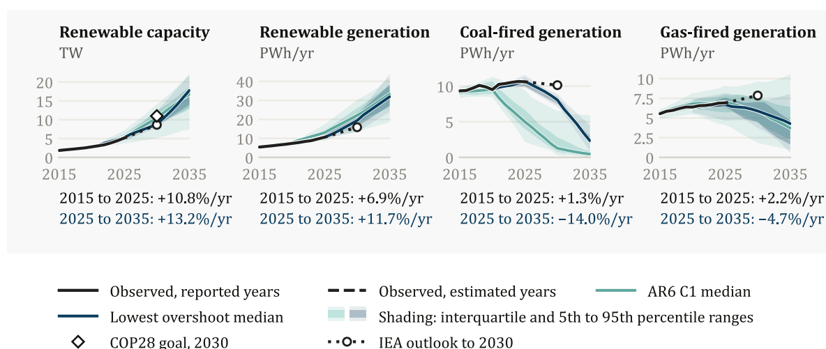
Figure 7b: Renewable capacity and renewable, coal-fired and gas-fired generation: observations, IEA outlooks to 2030, the COP28 tripling goal and the AR6 C1 and lowest-overshoot pathways, 2015–2035, drawn as in Figure 7a. Source: Byers et al. (2022); Riahi et al. (2026a); Ember (2026); IRENA (2026c); IEA (2025i, 2026a); UNFCCC (2024); Climate Resource calculations. 37
